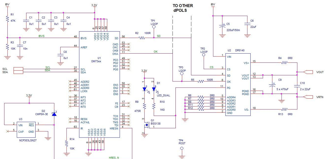
Figure 53. Typical Application with Digital Power Manager and I 2 C Interface
