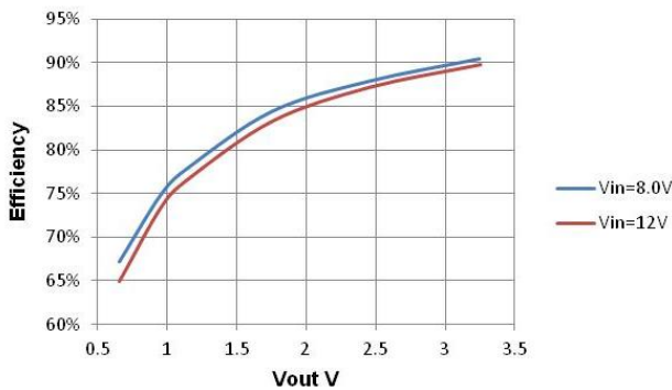
Figure 7. Efficiency vs V_{out} , Load=40A, F_{sw}=500kHz
