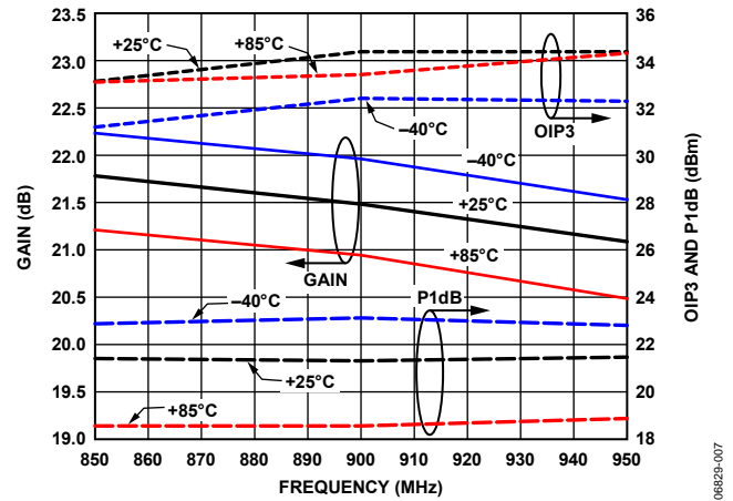
Figure 7. Gain, OIP3, and P1dB vs. Temperature
