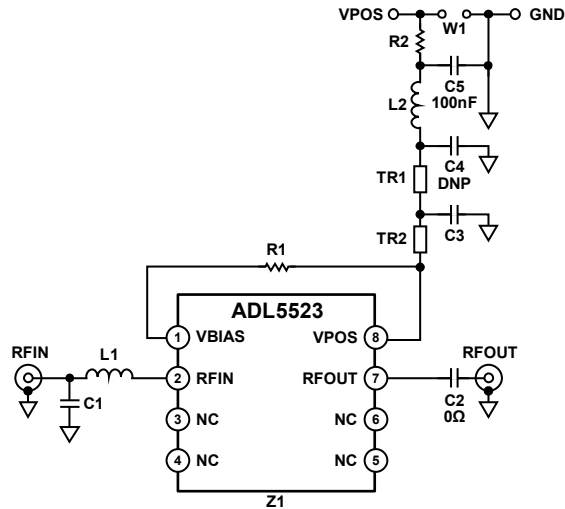
Figure 54. Evaluation Board Schematic
