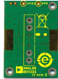
Figure 56. Evaluation Board Layout (Bottom View)
