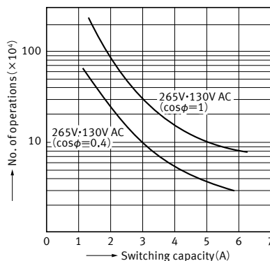
2-1. Switching life curve (1 Form A 1 Form B)
