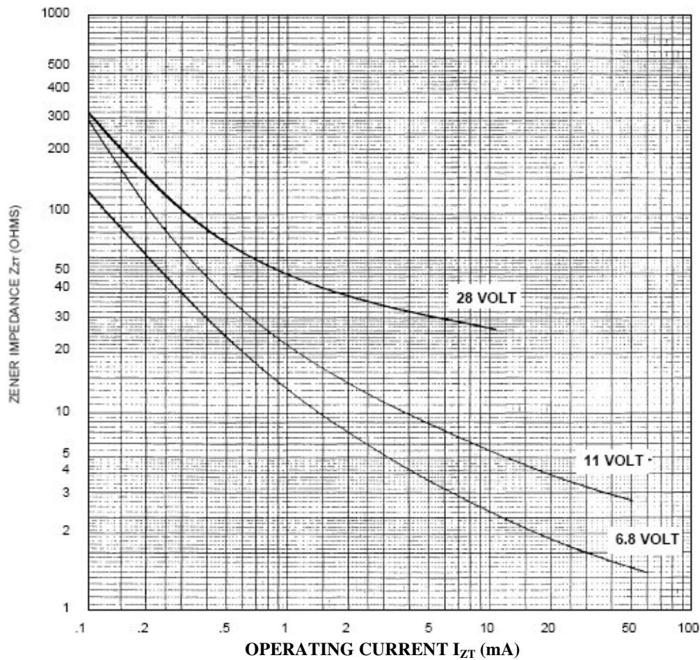
FIGURE 3 ZENER IMPEDANCE VS. OPERATION CURRENT
