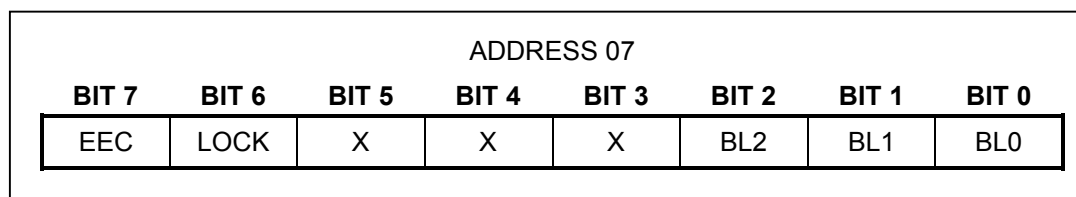
Figure 13. EEPROM Register Format
